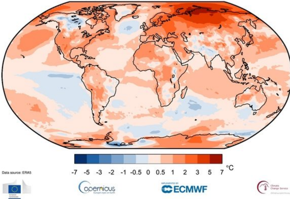
Temperature difference 2020 and 1981-2010
